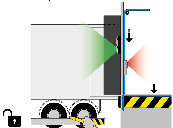
The COMBILOK® G 2 control panel indicator light turns green and signals that the vehicle is safely restrained by the G 2 . The leveller control panel indicator light also turns green indicating that the leveller is in position and loading or unloading can safely commence.
